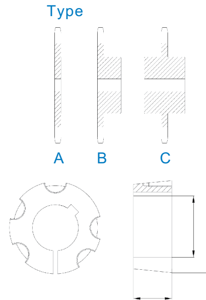
▼ Taper lock Bush
